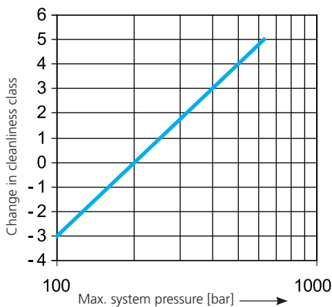
Figure 3: Influence of the operating pressure on required oil cleanliness
