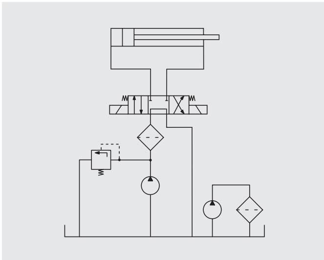
Hydraulic system with high-pressure filter and off-line filter unit
