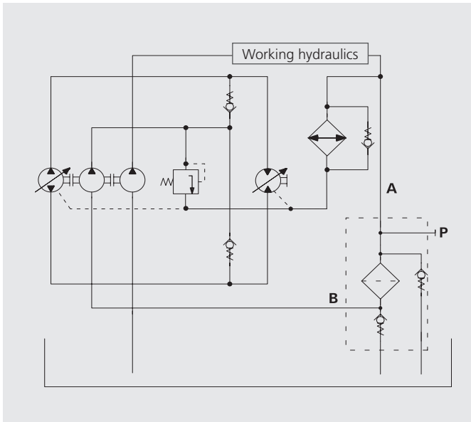
Figure 1: Hydraulic system with return-suction filter
