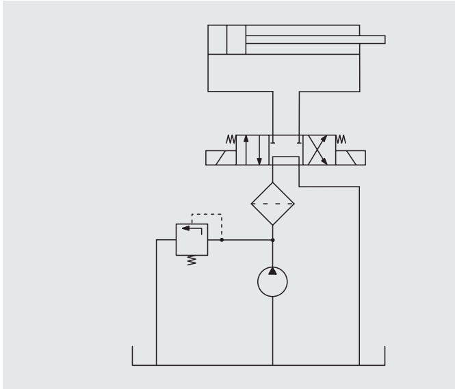
Figure 1: Hydraulic system with high-pressure filter
