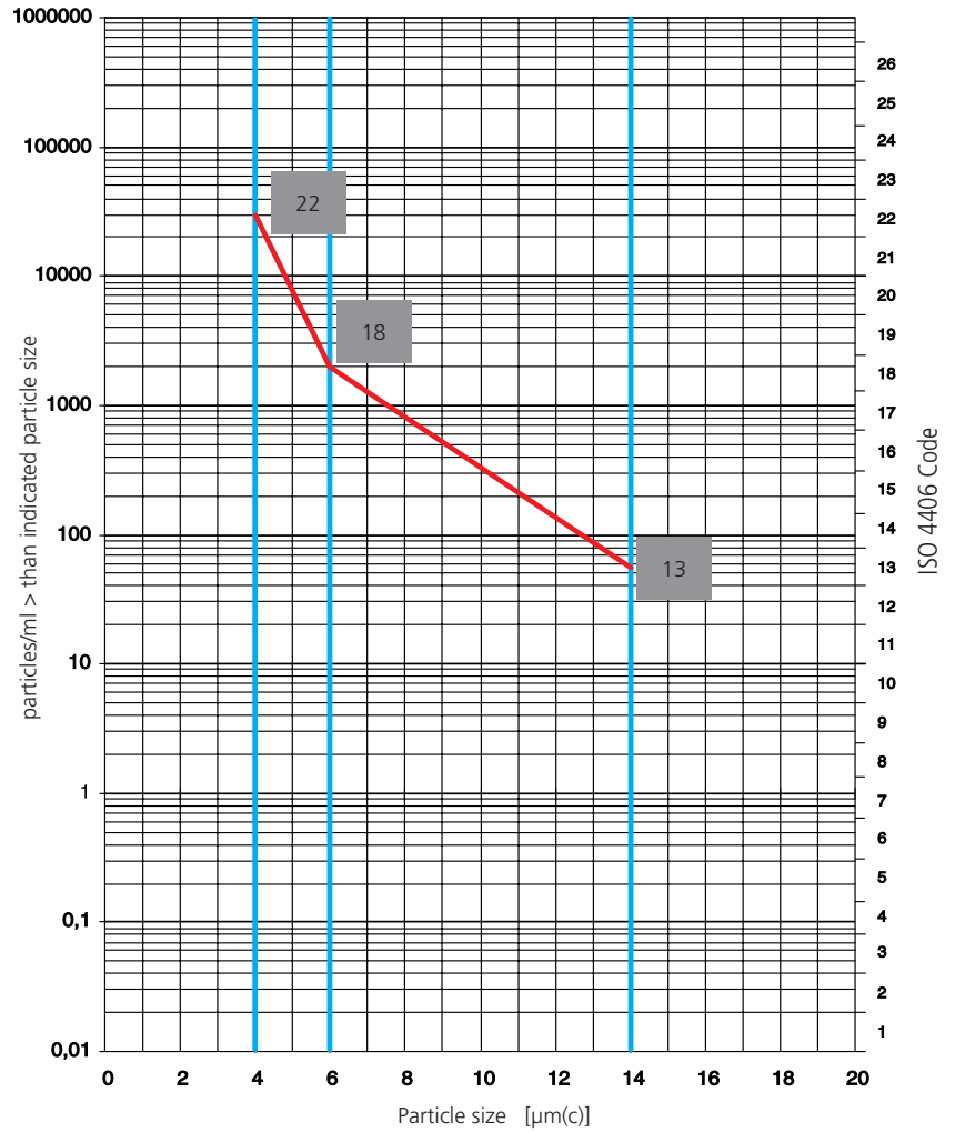
Evaluation of an oil sample according to ISO 4406:1999
