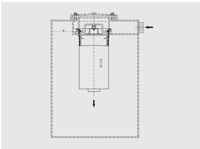
Figure 2: Return filter E 441 ... E 700 for installation in tanks
