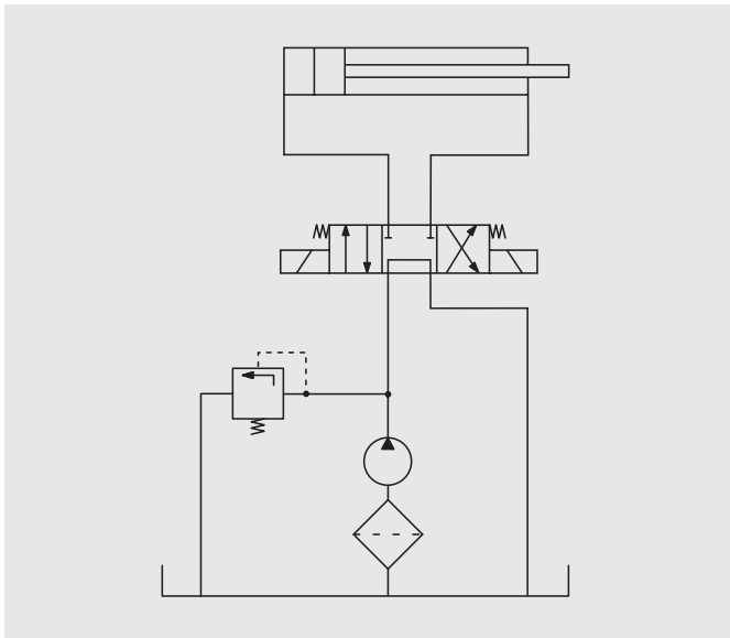
Figure 1: Hydraulic system with suction filter
