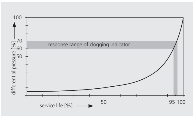
Typical progression of contamination of a filter element throughout its service life
