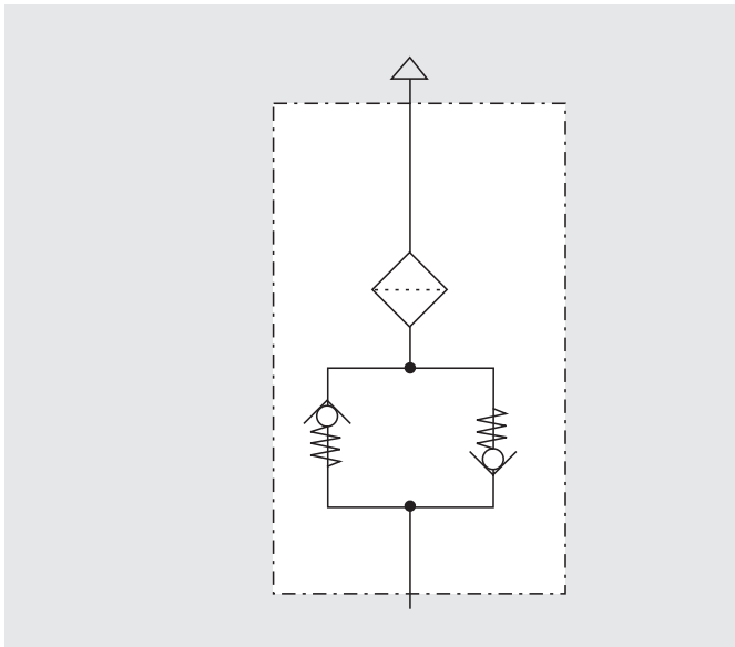
Figure 1: Circuit diagram for ventilating filters with double check valve
