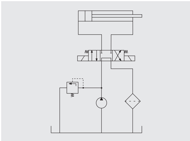
Figure 1: Hydraulic system with return filter
